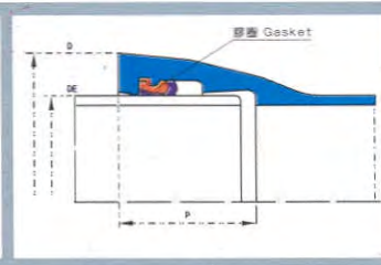
T型防滑脱接口 (T Type anti-thrust joint)
