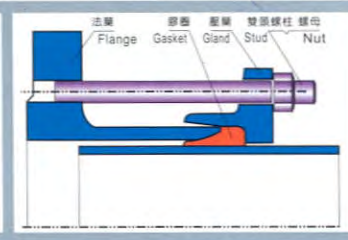
VJFA接口 (VJFA Joint)
