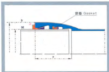
NT型防滑脱接口 (NT Type anti-thrust joint)
