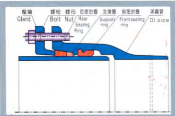
GTK高压城市燃气管接口 (GTK joint for high pressure urban combustion gas pipeline)
