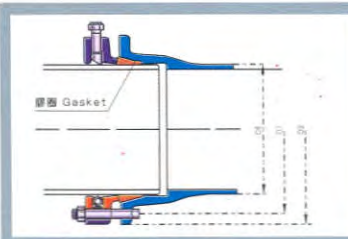
K型自锚式接口 (K Type self-anchored joint)
