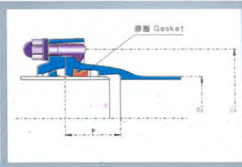
TF自锚式接口 (TF Type self-anchored joint)
