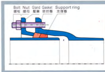
KFM自锚可拆卸接头 (KFM self-anchored dismantlable joint)
