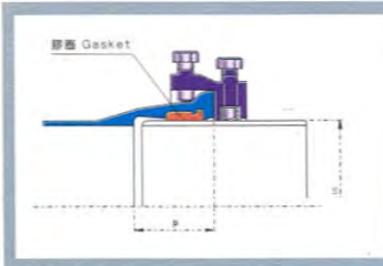
TJ自锚式接口 (TJ Type self-anchored joint)
