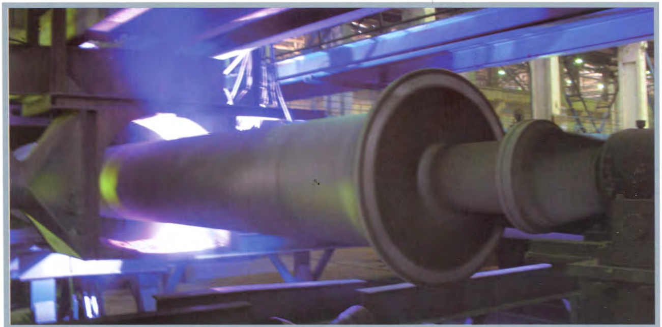
喷锌 Metallic zinc applying
